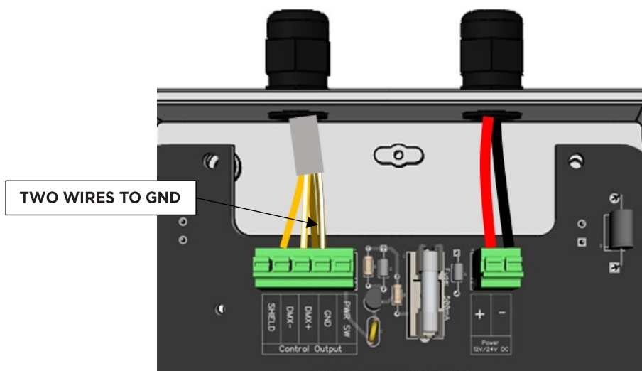
Figure 4: Pro Series Receiver wiring
