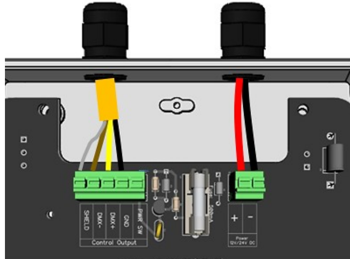
Figure 3: OceanConnect JB, 2-Way JB, Explore E6/E7 Receiver wiring (Note: red wire in control cable is not connected)
