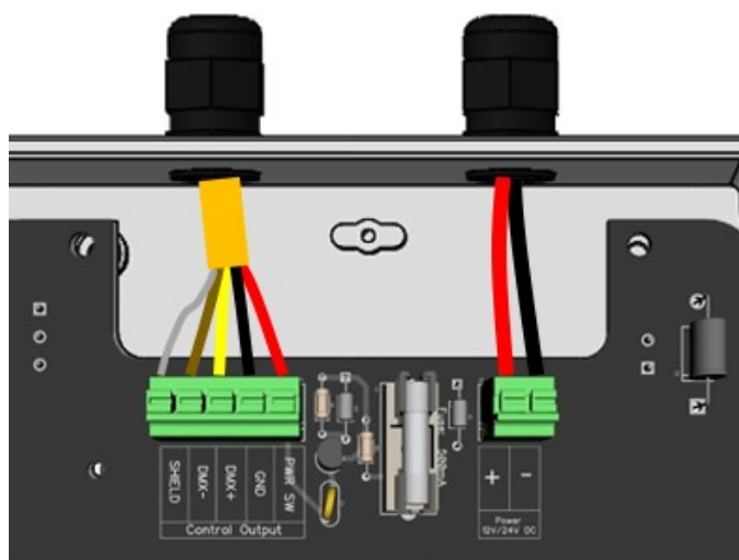
Figure 2: X-Series Receiver wiring
