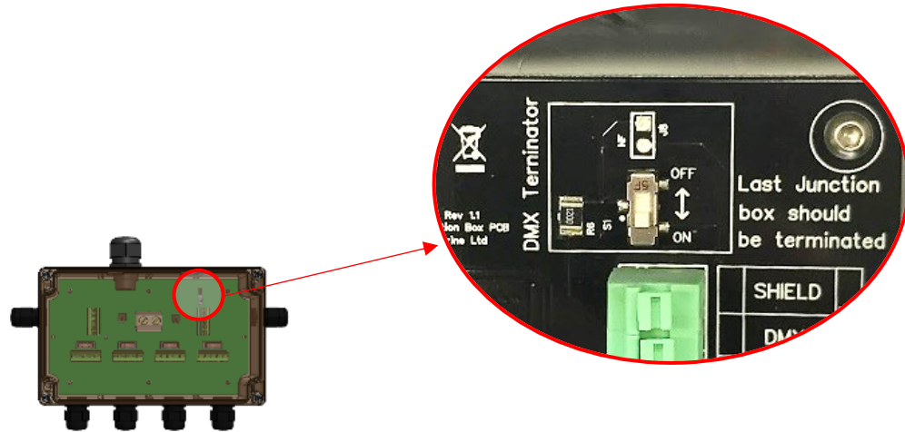
Figure 2: DMX Terminator switch
