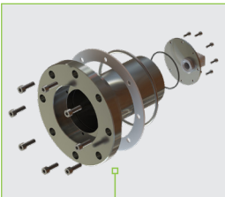
HYBRID WET-MATE INSTALLATION KIT
