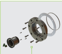
HYBRID DRY-MATE INSTALLATION KIT
